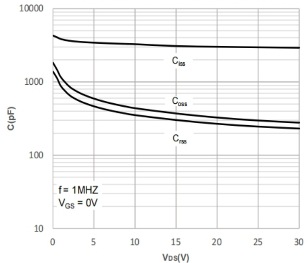
Figure 6: Capacitance Characteristics
